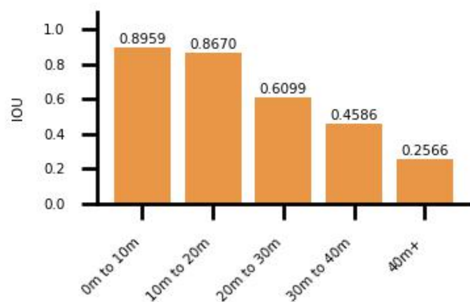
Distance vs. IOU for construction_vehicle
