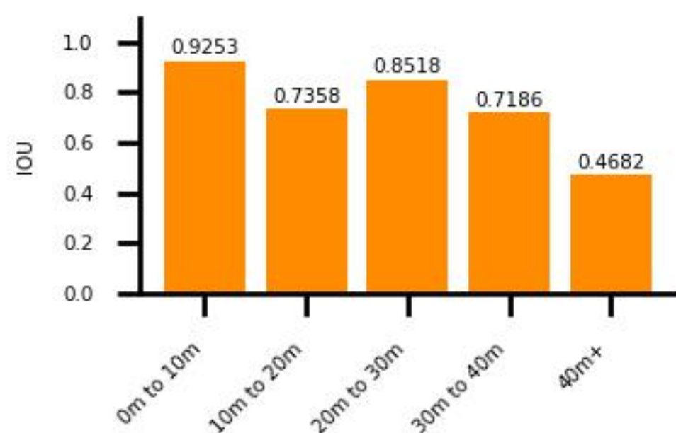
Distance vs. IOU for trailer
