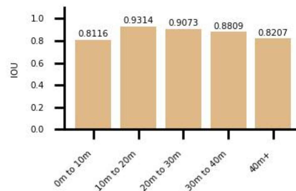
Distance vs. IOU for manmade
