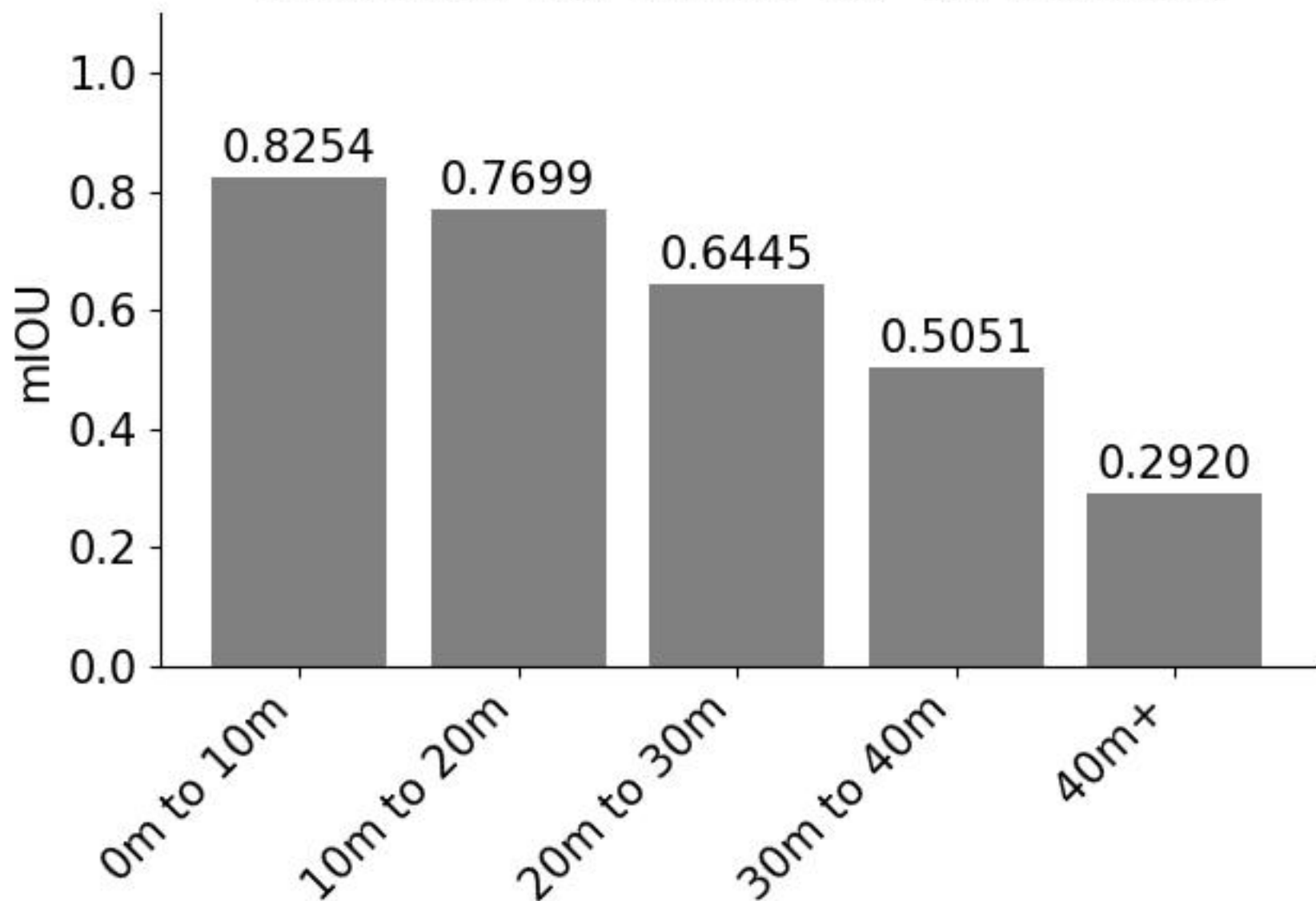
Distance vs. mIOU for all classes
