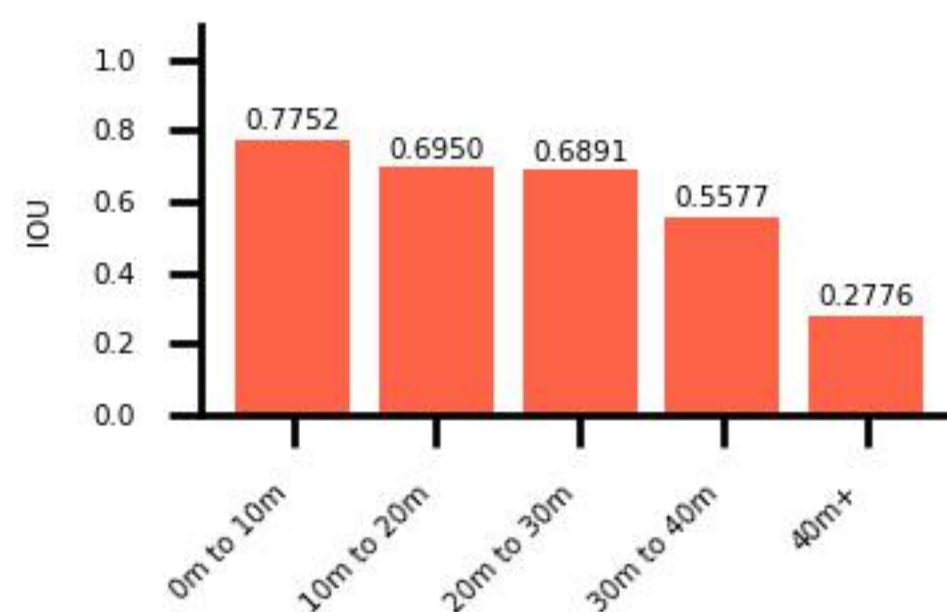
Distance vs. IOU for truck
