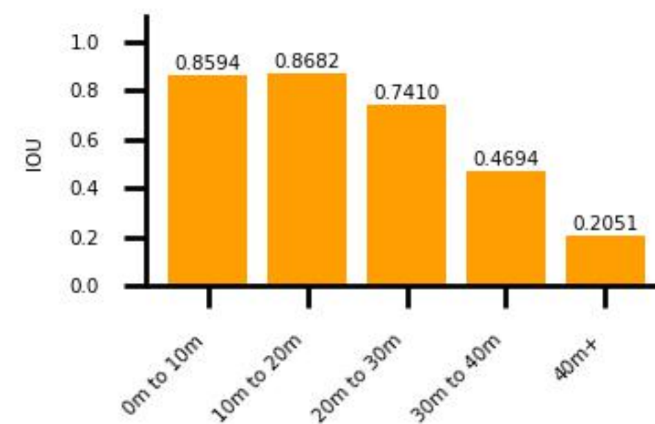
Distance vs. IOU for car
