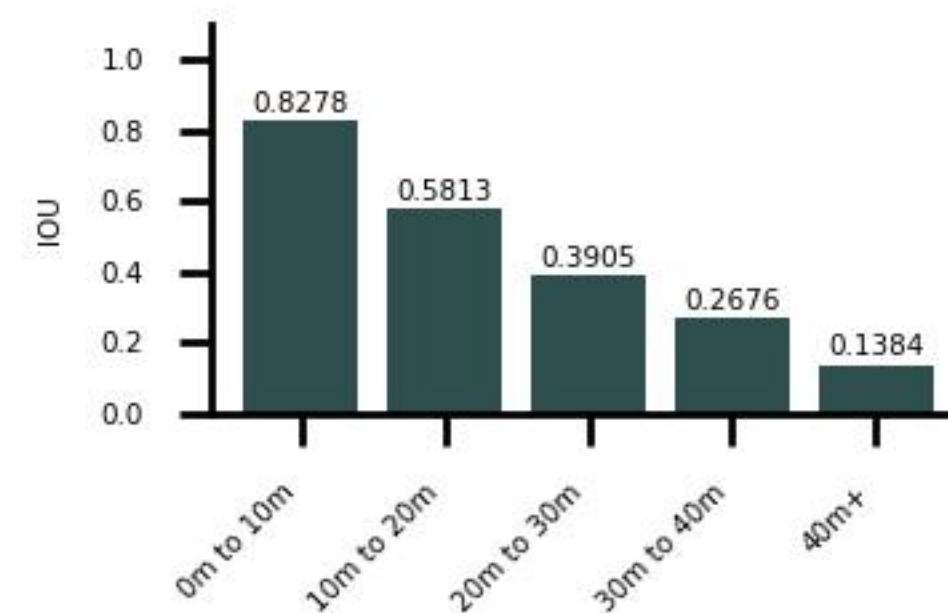
Distance vs. IOU for traffic_cone
