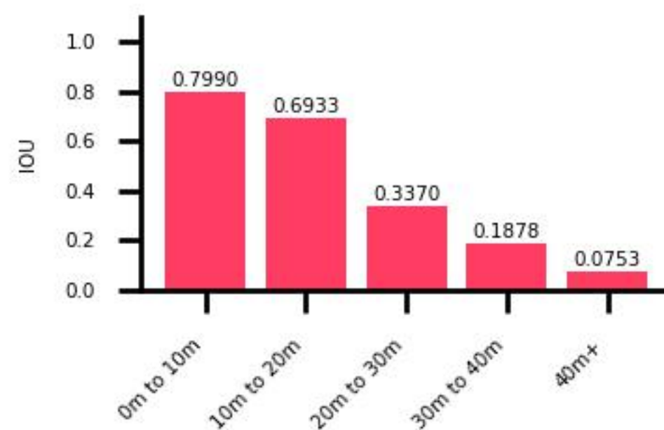
Distance vs. IOU for motorcycle
