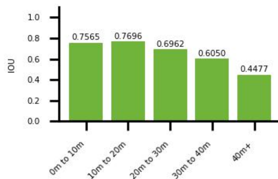
Distance vs. IOU for terrain
