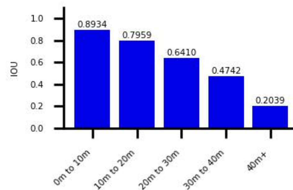
Distance vs. IOU for pedestrian
