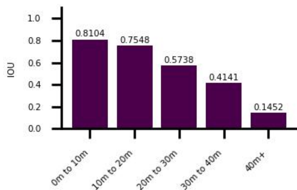
Distance vs. IOU for sidewalk
