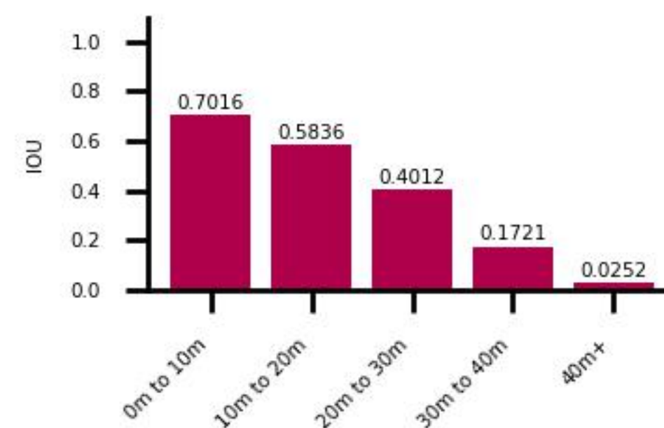
Distance vs. IOU for other_flat
