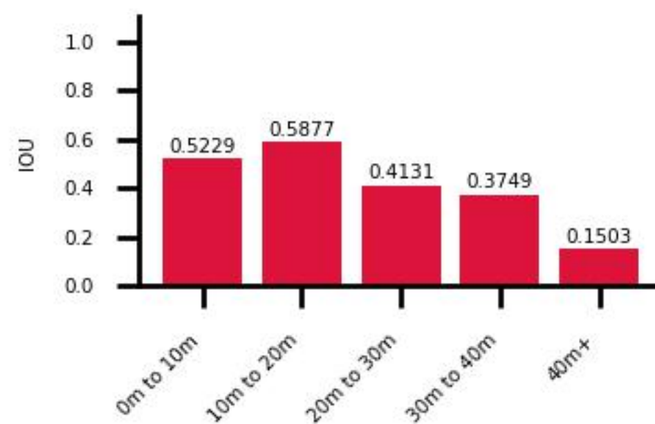
Distance vs. IOU for bicycle
