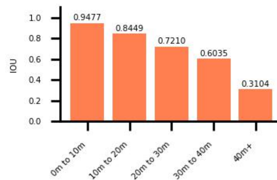
Distance vs. IOU for bus
