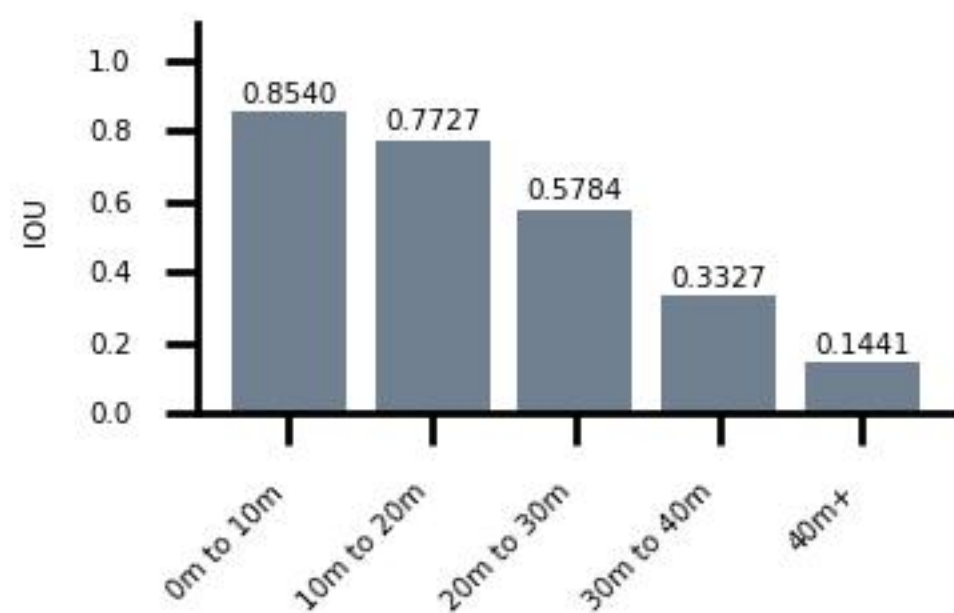
Distance vs. IOU for barrier
