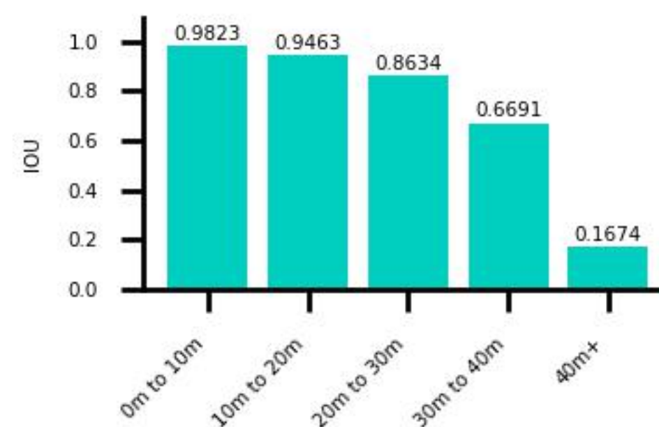
Distance vs. IOU for driveable_surface
